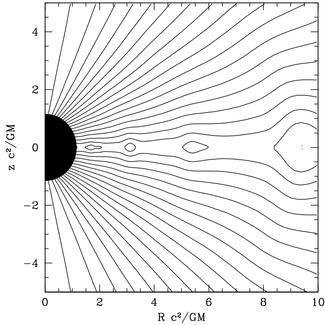
Fig. 1 A contour plot of the magnetic flux ( \Psi = RA_\phi ) showing the inner (cylindrical radius) R < 10GM/c^2 for the MHD a = 0.99 model described in the text. The structure of the magnetosphere relaxes to monopolar-like solution, as predicted by [7]. Note also the development of the tearing modes and the formation of magnetic islands in the equatorial current sheet.
